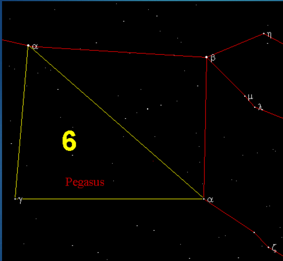
alpha And — gamma Peg — alpha Peg
